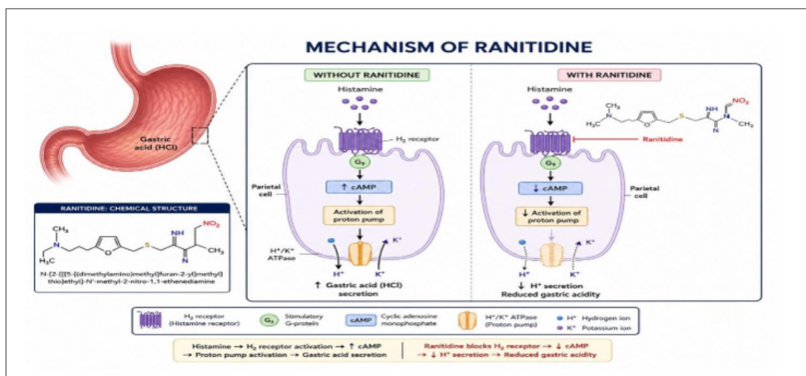
Figure 2. Mechanism of Ranitidine
