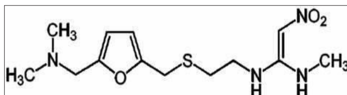
Figure 1. Chemical Structure of Ranitidine
