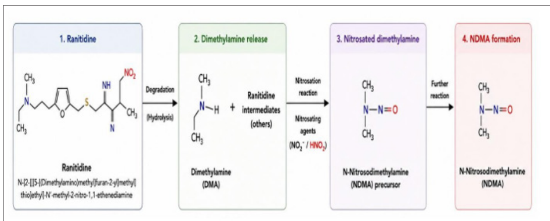
Figure 3. Mechanism of NDMA Formation
