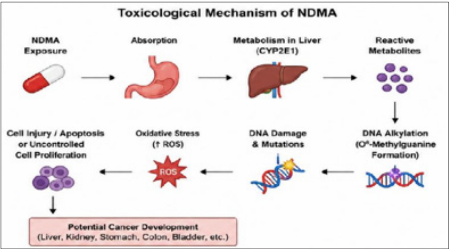
Figure 4.Toxicological Mechanism of NDMA
